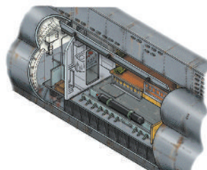
N72008 (1/72) U-boat VII Winding platform (2 chute version)
