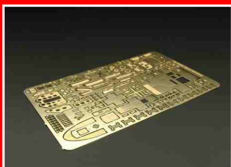
BRL32017 Kawanishi N1K2-J Shiden Kai PE set for HASEGAWA kit
